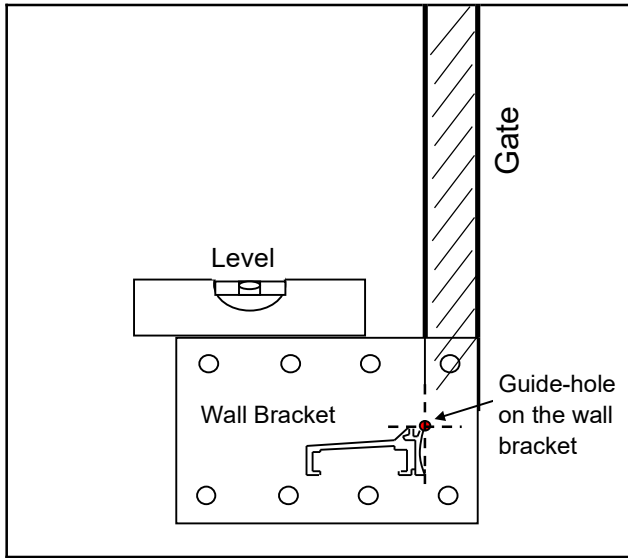
Alignment of wall bracket guide-hole with the marking point
