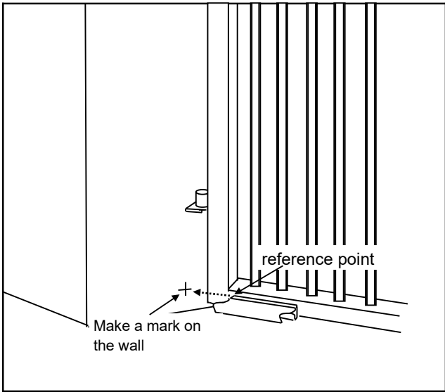
Make a mark on the wall by using the C-channel+base plate
