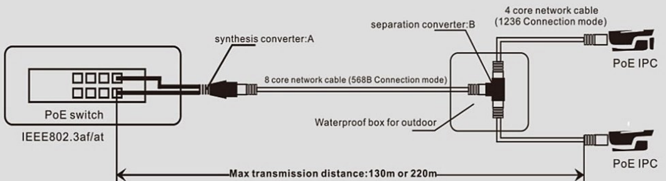
Installation diagram: Model: GNT-5313AB
