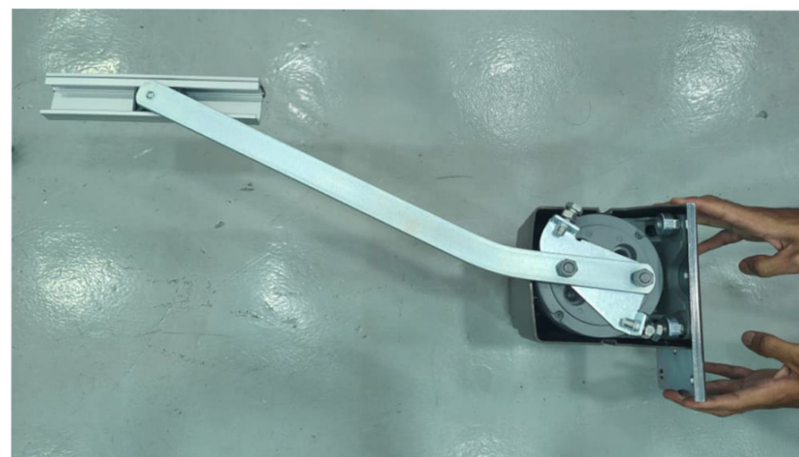
Right Motor Bottom View
